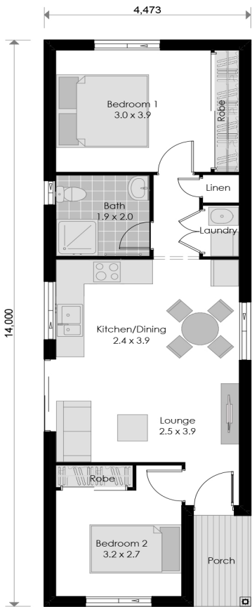
FLOOR PLAN
