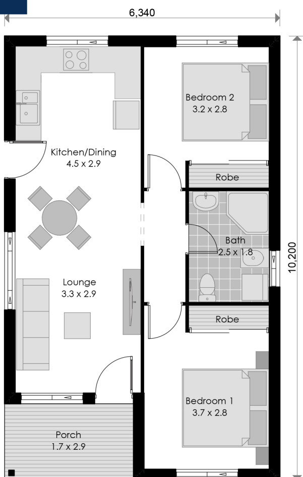
FLOOR PLAN
