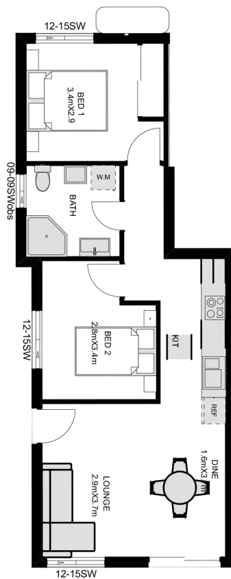
FLOOR PLAN
