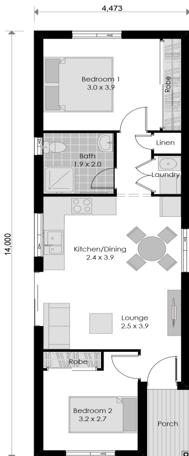
FLOOR PLAN
